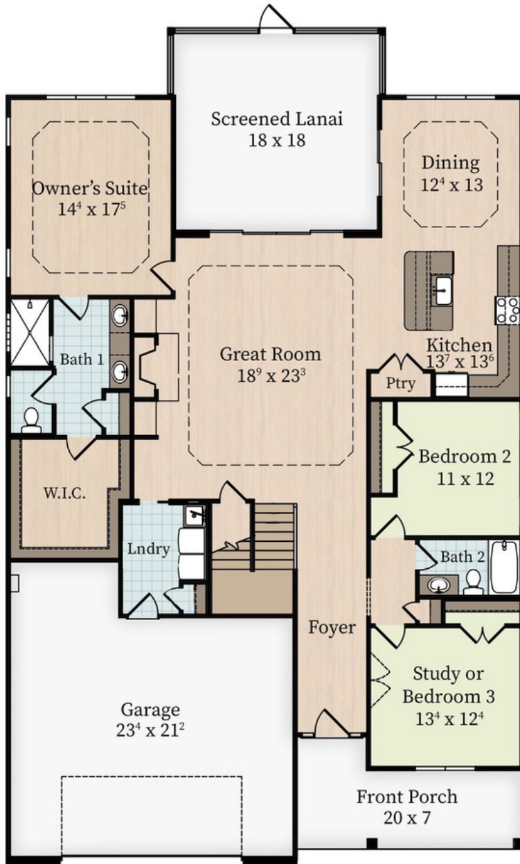
First Floor
